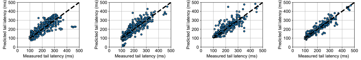
(a) Linear regression with Pod CPU. (b) Linear regression with Pod CPU and VM CPI. (c) Neural network with Pod CPU. (d) Neural network with Pod CPU and VM CPI.
