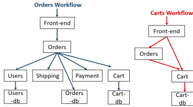
Fig. 2: Workflow DAGs.
